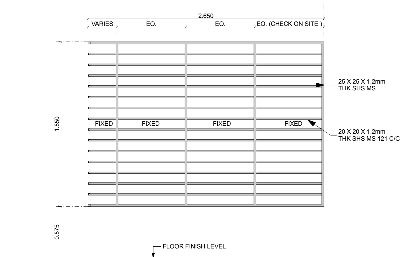
ELEVATION SCALE 1:25
