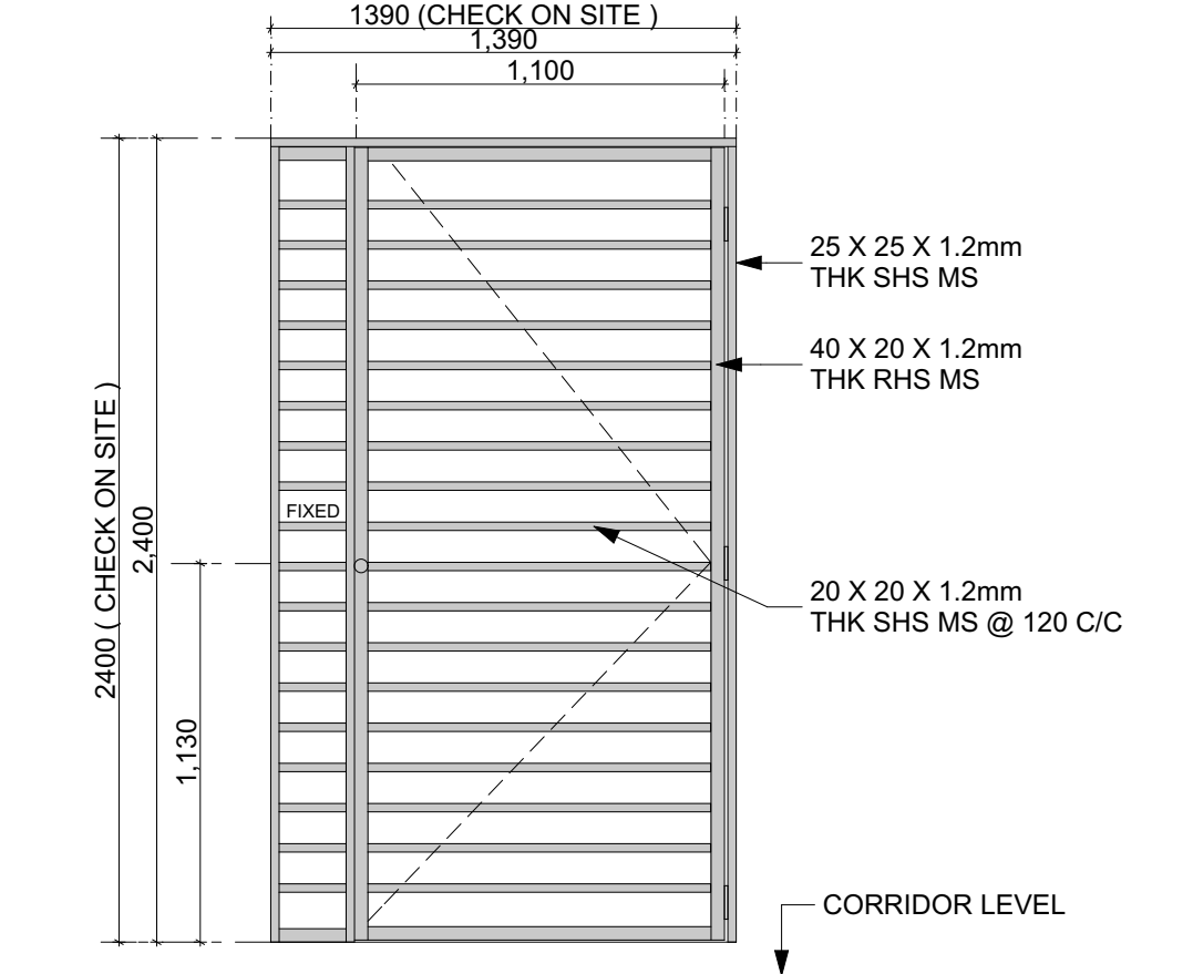
ELEVATION SCALE 1:20
